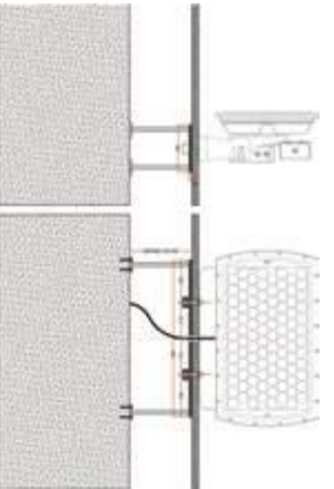
Detail
