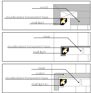
Section Detail
